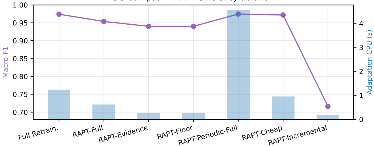
5G Campus — RAPT efficiency ablation
